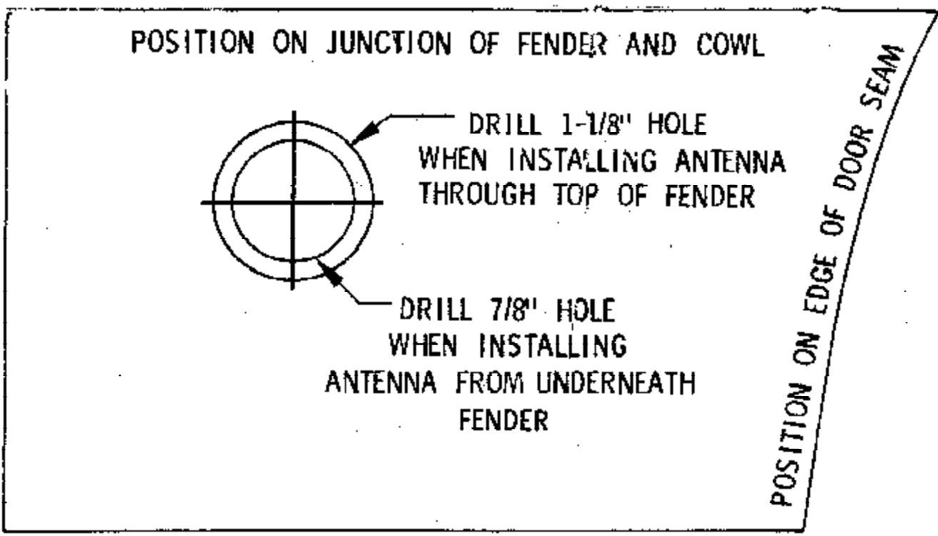
DRILL TEMPLATE FOR RETRACTABLE ANTENNA KARMANN GHIA
